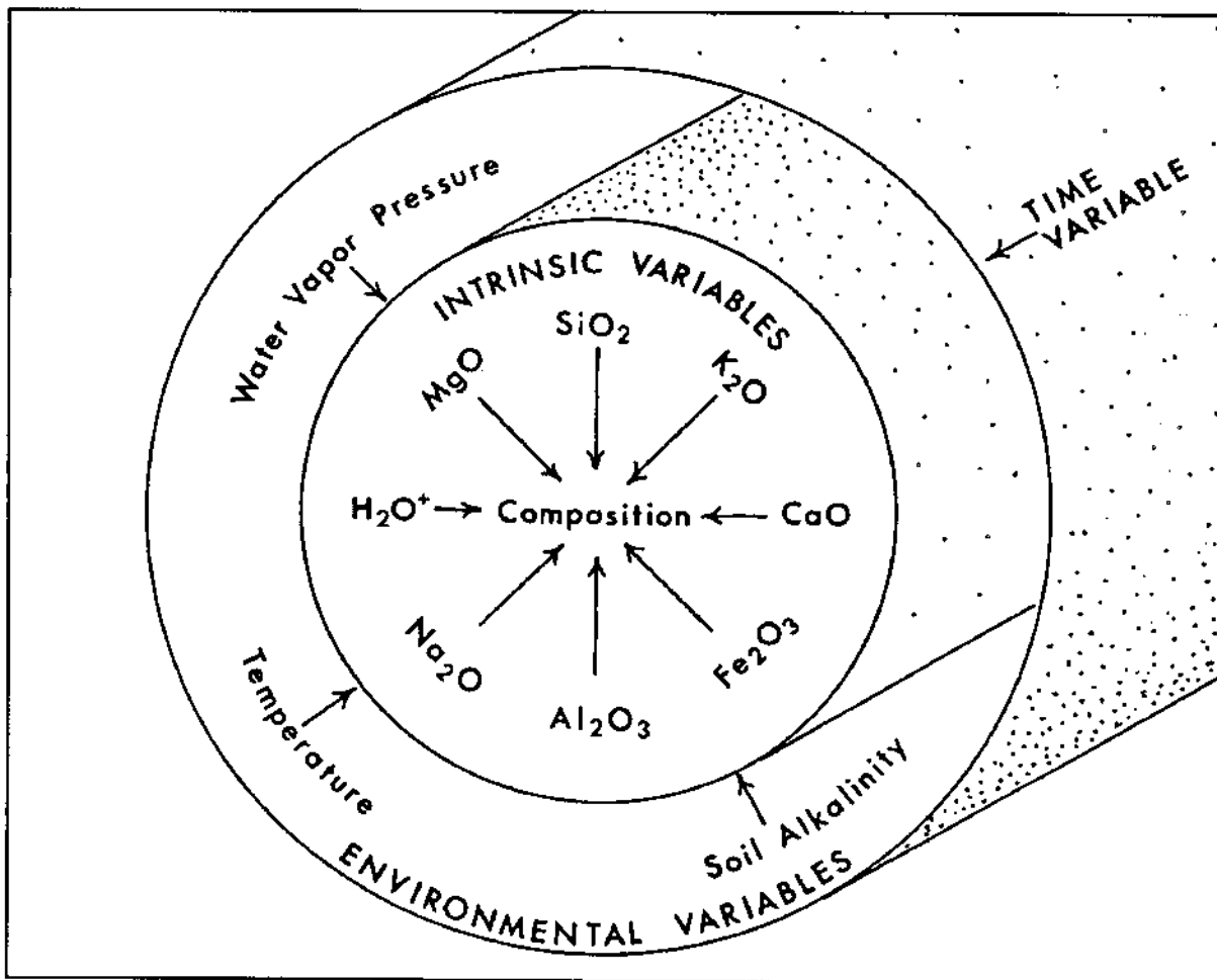
Figure 5-2 Major variables affecting the rate of hydration (from Skinner 1983:45).
