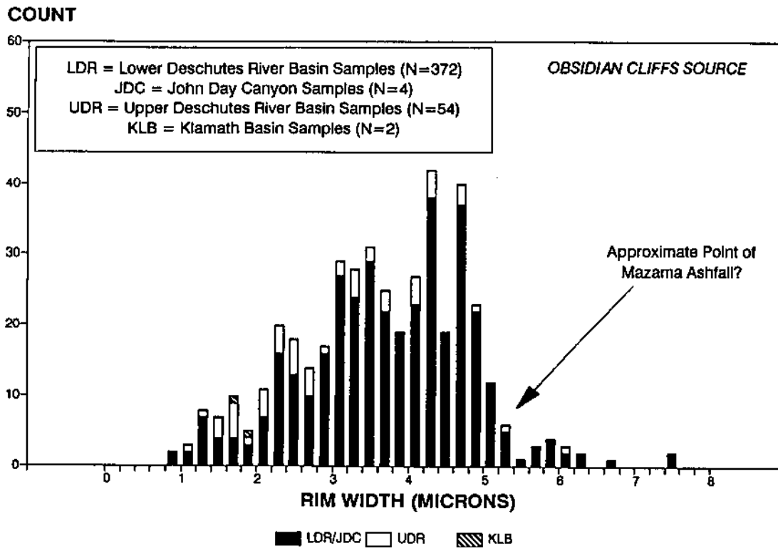
Figure 5-15 Frequency distribution of obsidian hydration rim measurements from artifacts correlated with the Obsidian Cliffs source.
