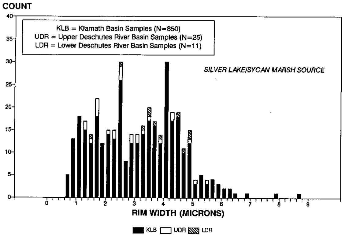
Figure 5-17 Frequency distribution of obsidian hydration rim measurements from artifacts correlated with the Silver Lake/Sycan Marsh source.
