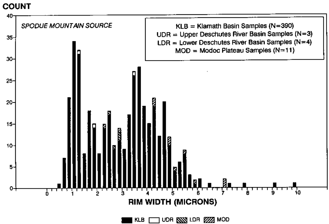
Figure 5-18 Frequency distribution of obsidian hydration rim measurements from artifacts correlated with the Spodue Mountain source.
