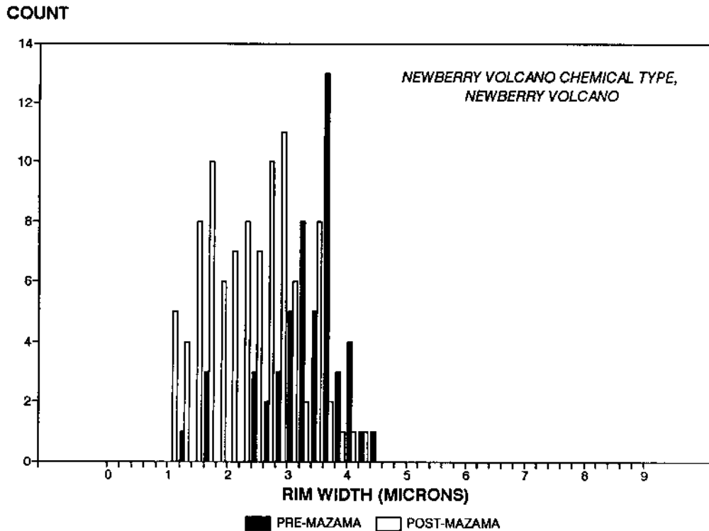
Figure 5-6 Frequency distribution of hydration rim values for pre- and post-Mazama artifacts from sites 35-DS-263 and 35-DS-557 that were correlated with the Newberry Volcano chemical group.
