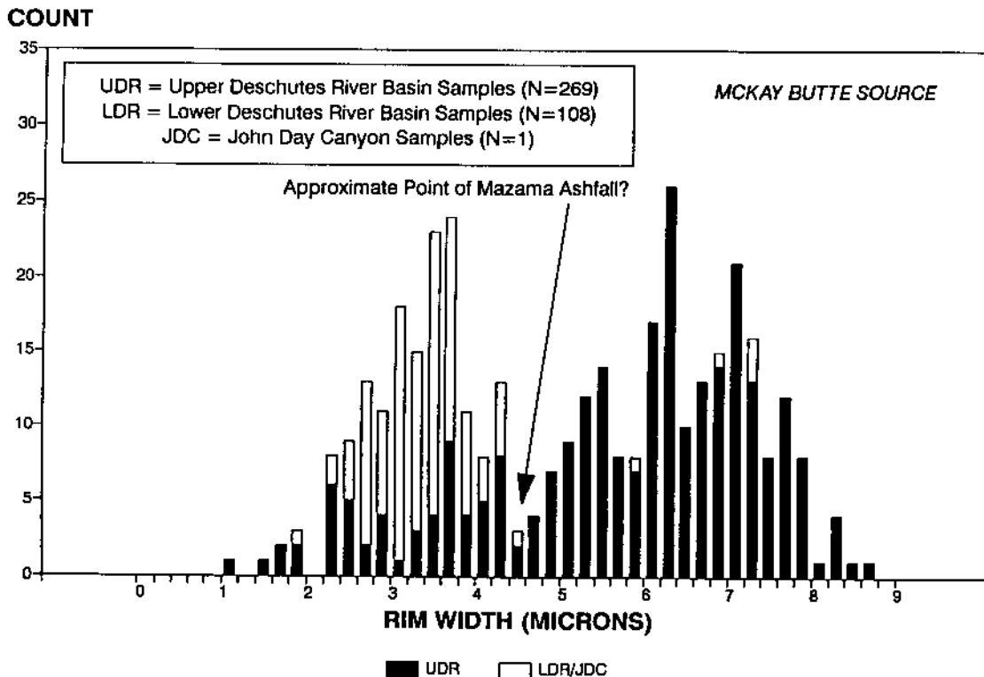
Figure 5-13 Frequency distribution of obsidian hydration rim measurements from artifacts correlated with the McKay Butte source.
