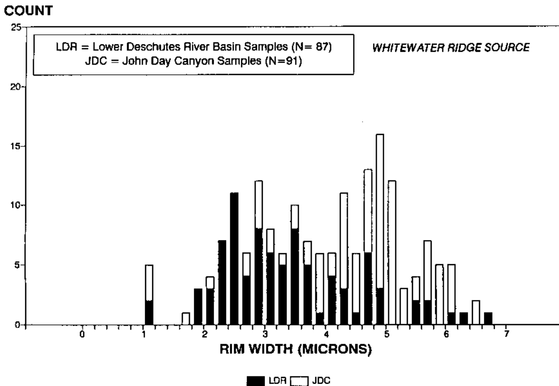
Figure 5-20 Frequency distribution of obsidian hydration rim measurements from artifacts correlated with the Whitewater Ridge source.
