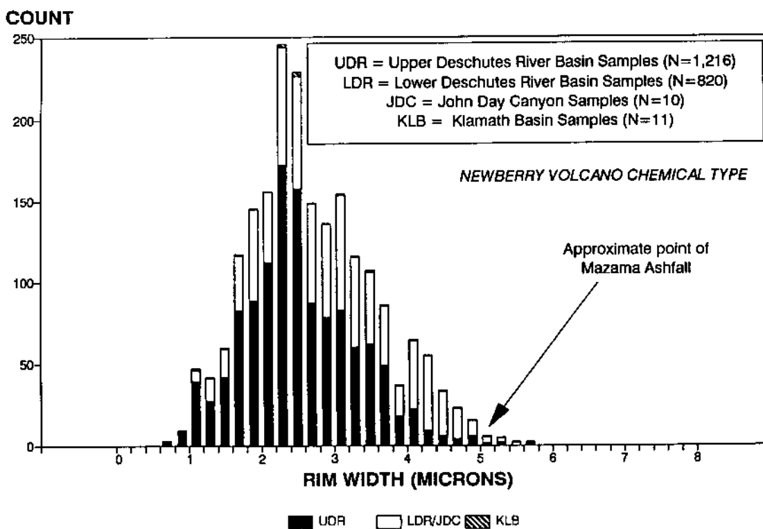
Figure 5-14 Frequency distribution of obsidian hydration rim measurements from artifacts correlated with the Newberry Volcano chemical group.
