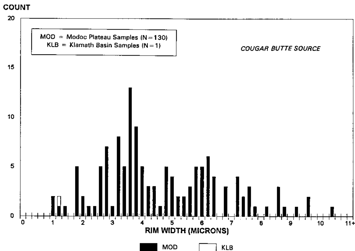
Figure 5-21 Frequency distribution of obsidian hydration rim measurements from artifacts correlated with the Cougar Butte source.
