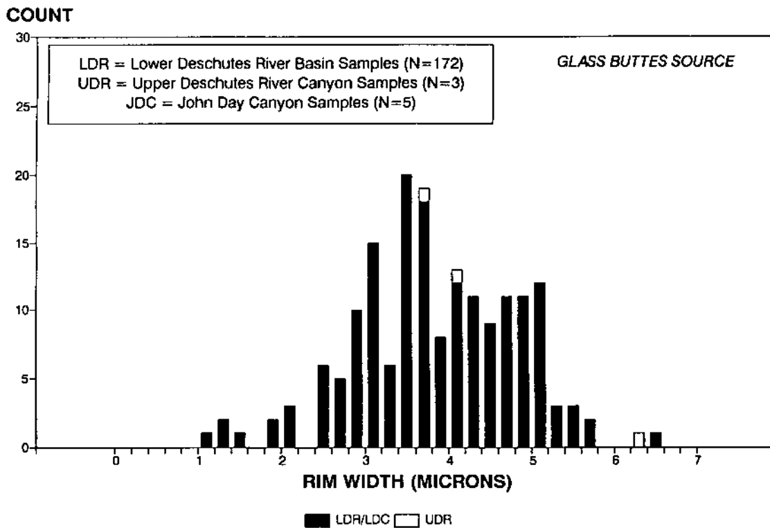
Figure 5-12 Frequency distribution of obsidian hydration rim measurements from artifacts correlated with the Glass Buttes source.
