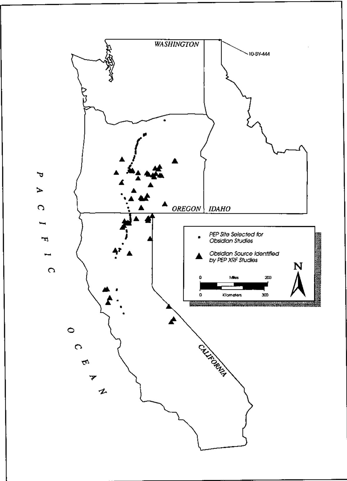
Figure 5-1 Distribution of Project sites selected for obsidian hydration studies.
