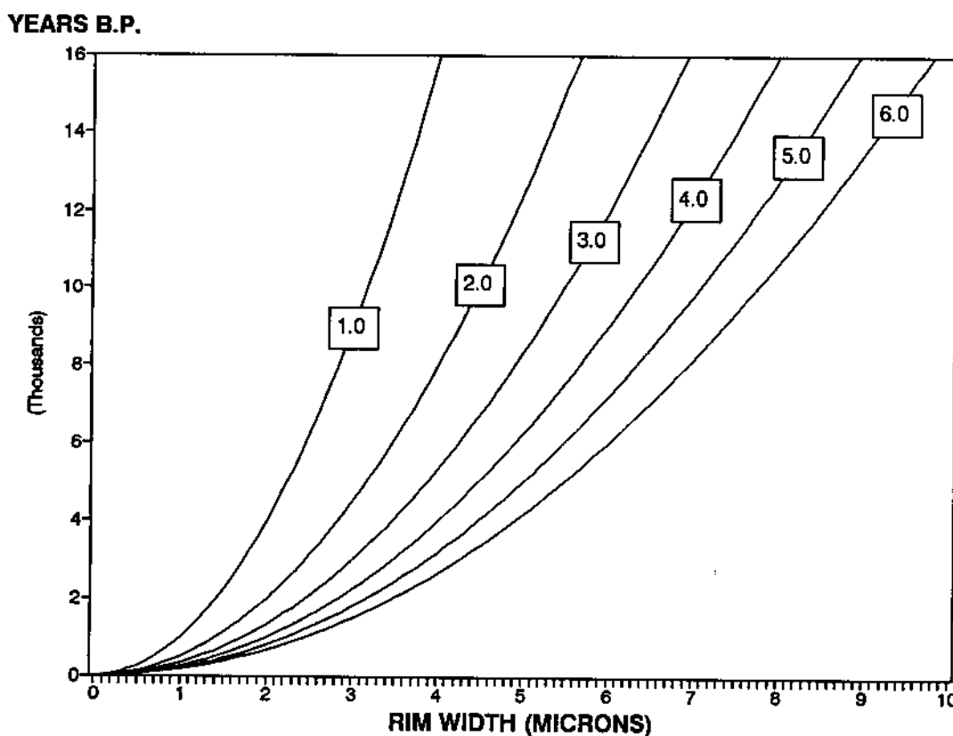
Figure 5-3 Examples of the results of different hydration rates applied to the diffusion model ( x^2=kt ) of hydration developed by Friedman and his associates. (1.0 = rate of 1 \mu\text{m}^2 / 1,000 years, and so on).
