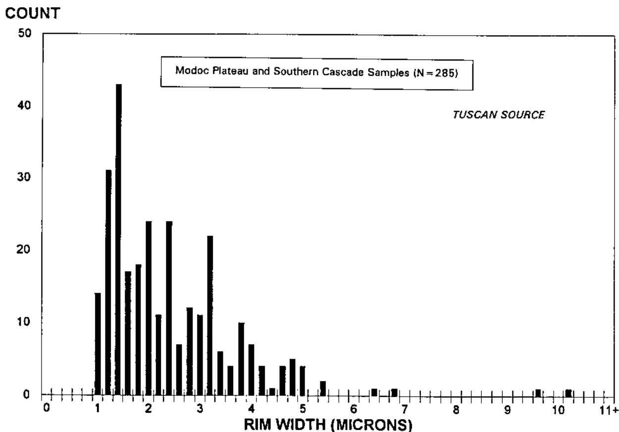
Figure 5-24 Frequency distribution of obsidian hydration rim measurements from artifacts correlated with the Tuscan source.
