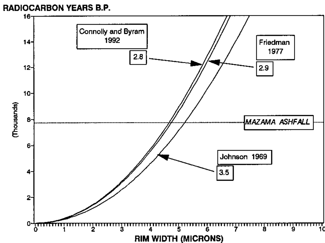
Figure 5-9 Published and proposed obsidian hydration rates for selected sources. (The numbers refer to rates in \mu\text{m}^2/1,000 years, e.g., 2.9 \mu\text{m}^2/1,000 years).
