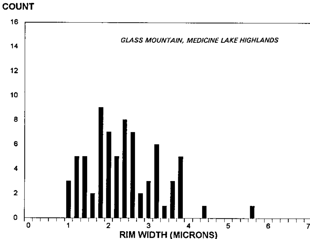
Figure 5-8 Frequency distribution of hydration rim values for samples correlated with the Glass Mountain source.
