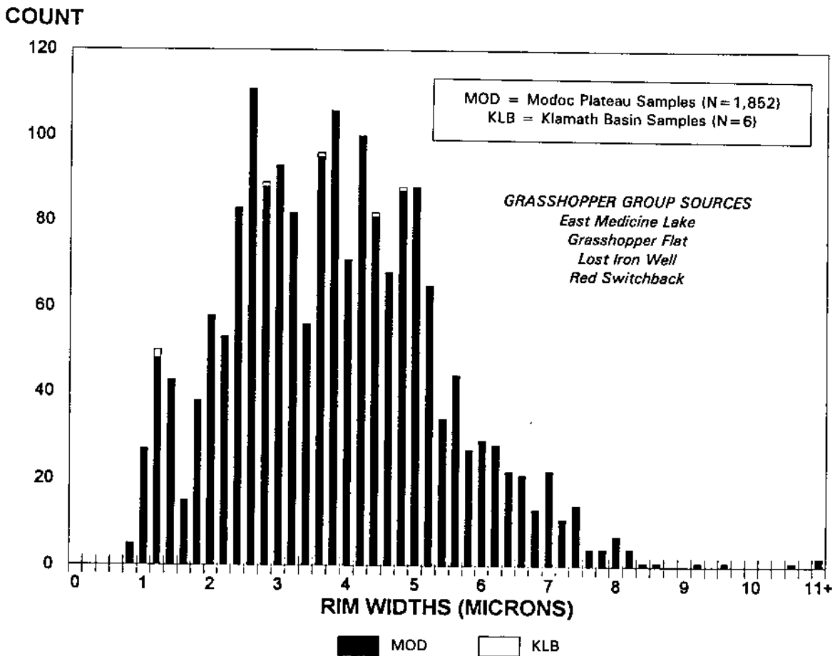
Figure 5-22 Frequency distribution of obsidian hydration rim measurements from artifacts correlated with the Grasshopper Group chemical source.
