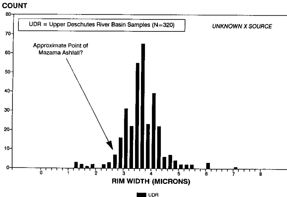
Figure 5-19 Frequency distribution of obsidian hydration rim measurements from artifacts correlated with the Unknown X source.
