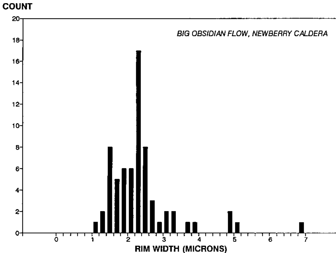
Figure 5-5 Frequency distribution of hydration rims associated with Big Obsidian Flow chemical group artifacts.
