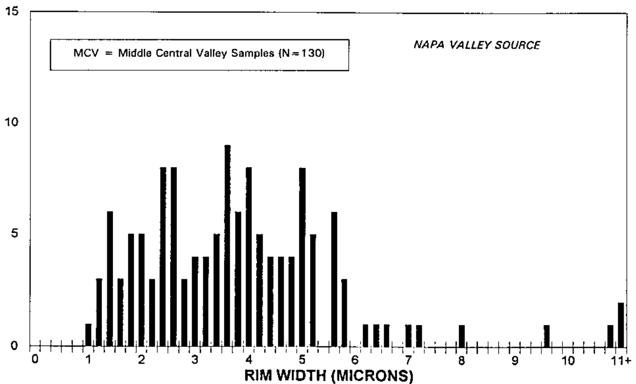
Figure 5-23 Frequency distribution of obsidian hydration rim measurements from artifacts correlated with the Napa Valley chemical source.
