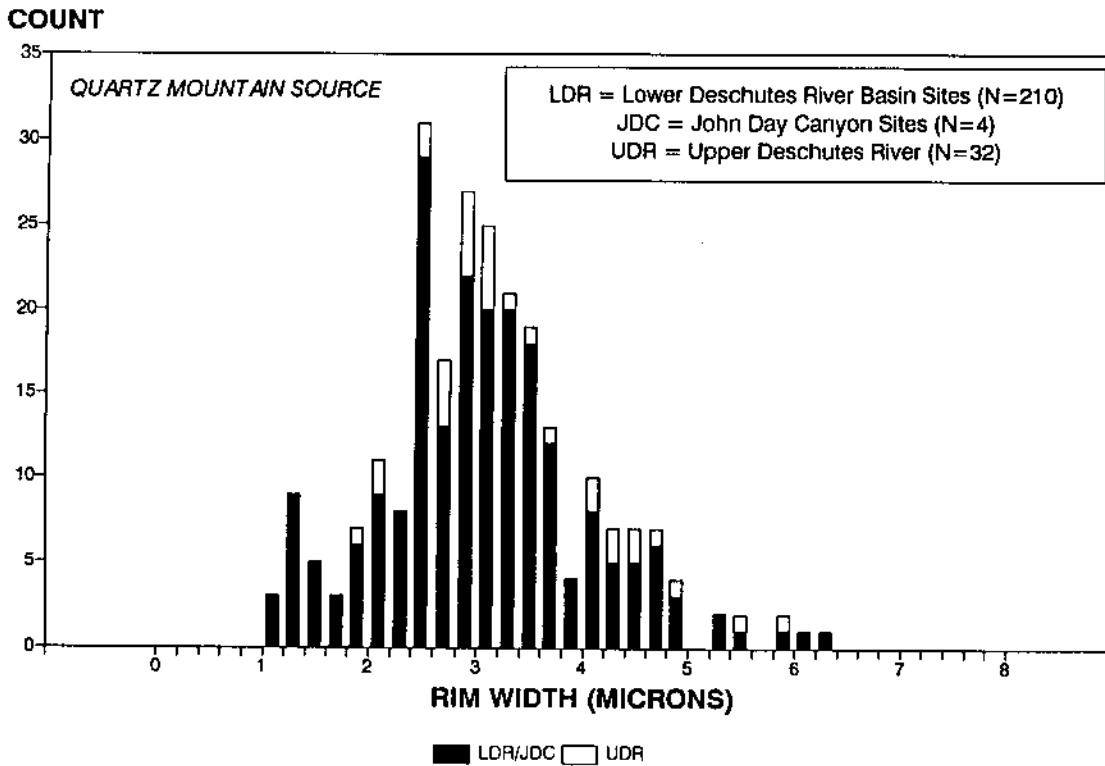
Figure 5-16 Frequency distribution of obsidian hydration rim measurements from artifacts correlated with the Quartz Mountain source.
